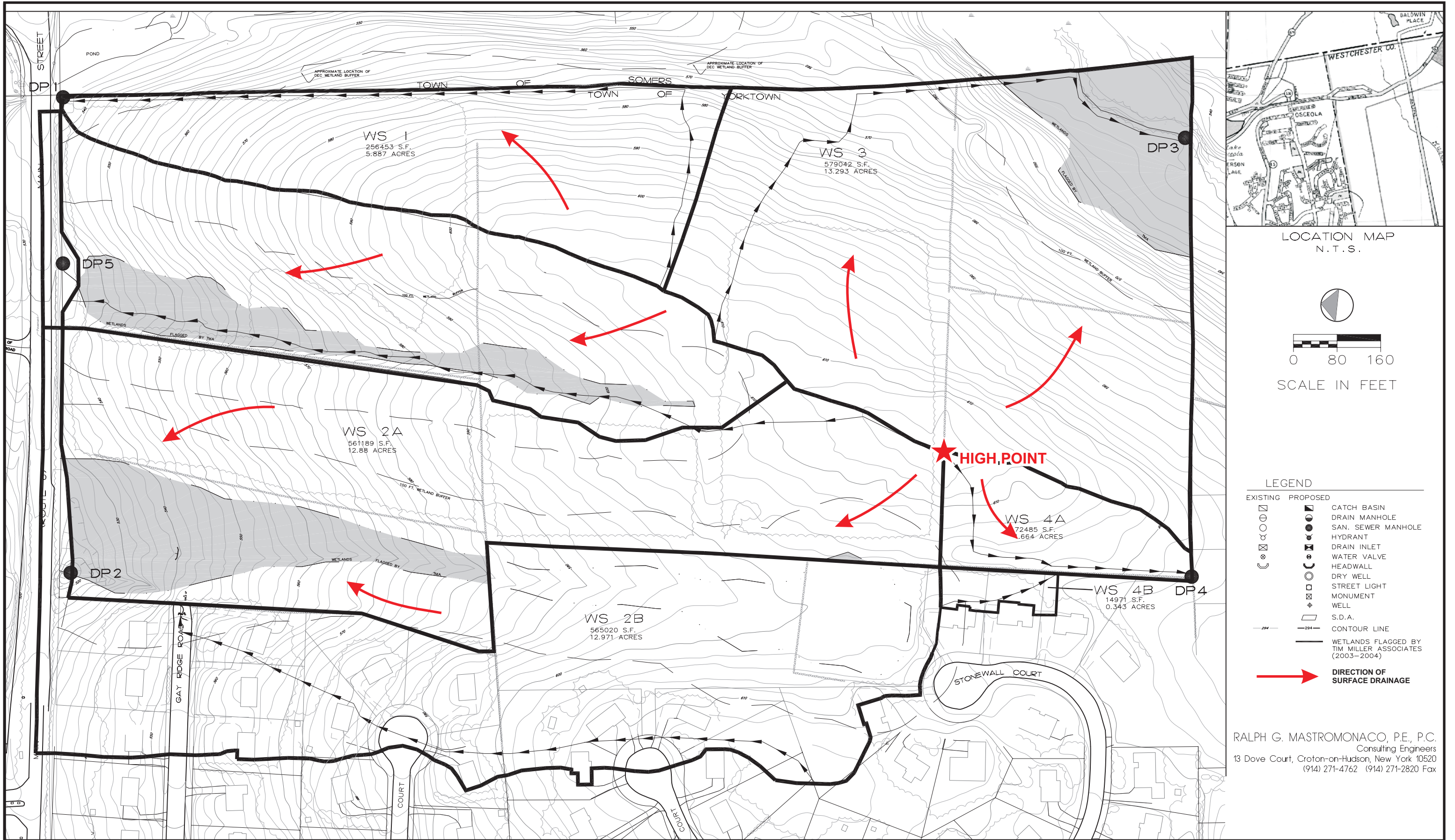
Figure 3.6-1: Existing Drainage Areas Yorktown Farms Subdivision Town of Yorktown, Westchester County, New York Source: Ralph G. Mastromonaco, P.E., P.C., 7/07 Scale: As shown
