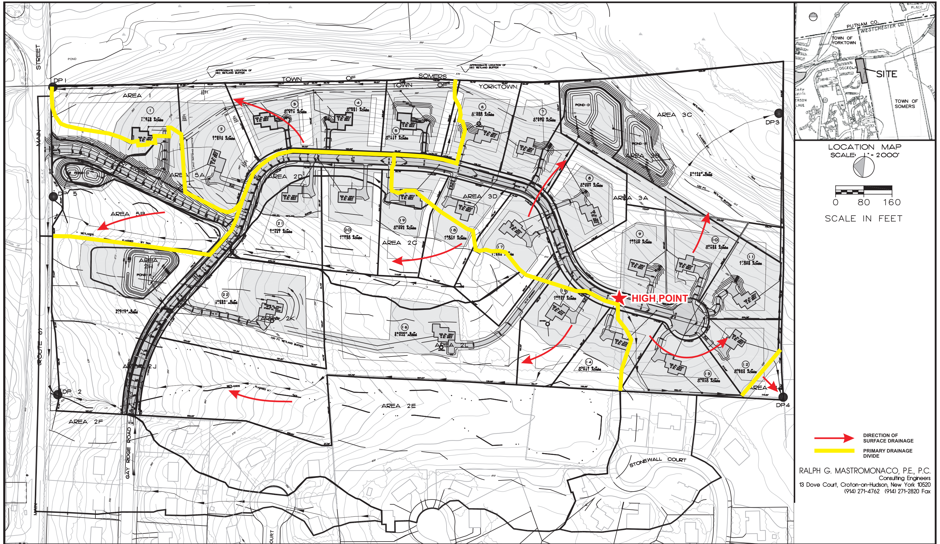
Figure 3.6-2: Post-Development Drainage Areas Yorktown Farms Subdivision Town of Yorktown, Westchester County, New York Source: Ralph G. Mastromonaco, P.E., P.C., 7/07 Scale: As shown
