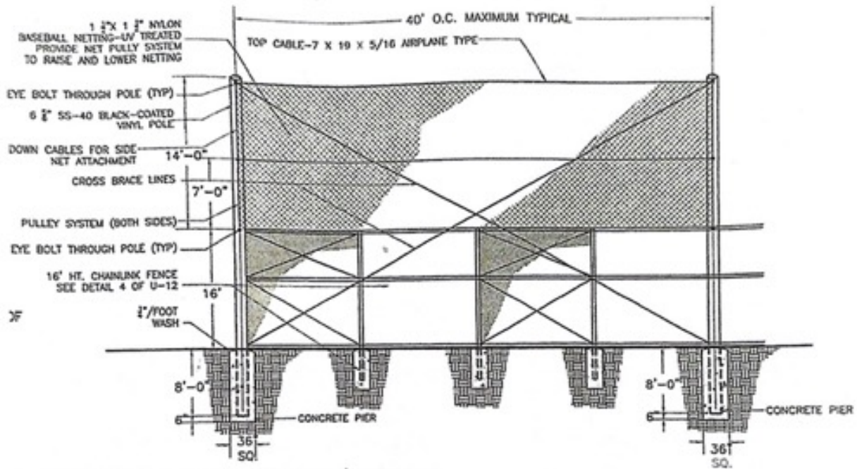
4 16' CHAINLINK FENCE W/ NETTING VI-119 NOT TO SCALE
